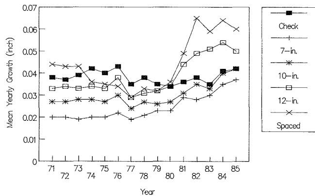
Figure 2—Radial growth of lodgepole pine before (1971 to 1980) and after (1981 to 1985) partial cutting treatments, East Long Creek, Shoshone National Forest, WY.
